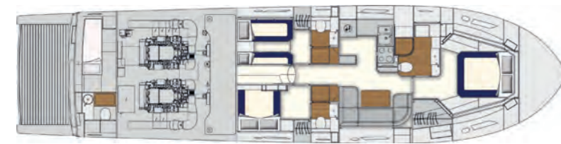
Lower Deck
